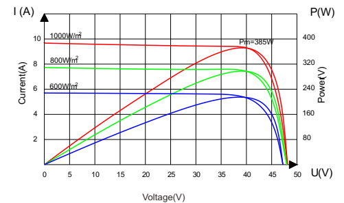
Current-Voltage&Power-Voltage Curve(385W)
