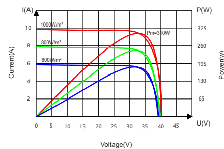
Current-Voltage&Power-Voltage Curve(310W)
