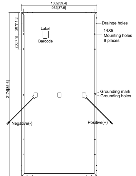
(Back side) Note:mm[inch]
