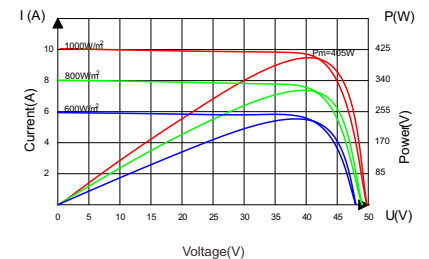
Current-Voltage&Power-Voltage Curve(405W)
