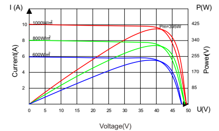
Current-Voltage&Power-Voltage Curve(395W)
