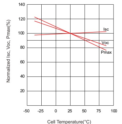
Temperature Dependence of Isc, Voc, Pmax(°C)
