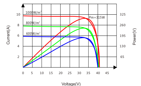
Current-Voltage&Power-Voltage Curve(315W)
