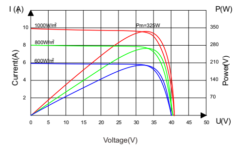
Current-Voltage&Power-Voltage Curve(325W)
