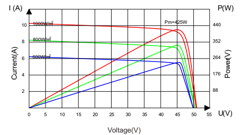
Current-Voltage&Power-Voltage Curve(425W)
