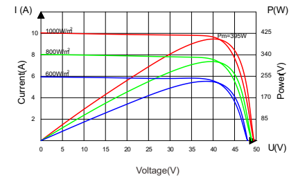
Current-Voltage&Power-Voltage Curve(395W)
