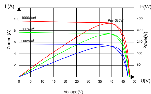
Current-Voltage&Power-Voltage Curve(385W)
