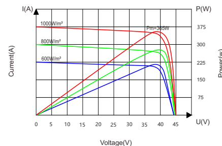
Current-Voltage&Power-Voltage Curve(365W)
