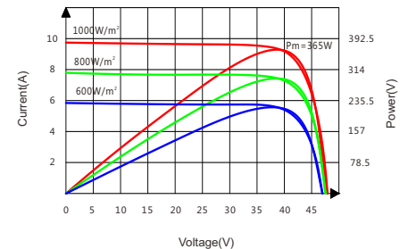
Current-Voltage&Power-Voltage Curve(365W)
