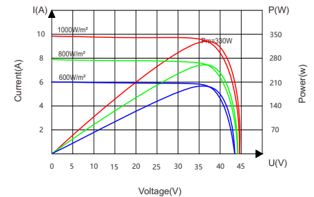
Current-Voltage&Power-Voltage Curve(330W)
