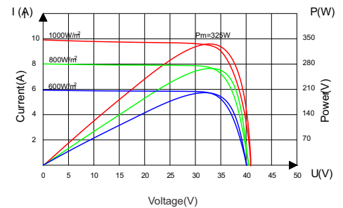
Current-Voltage&Power-Voltage Curve(325W)
