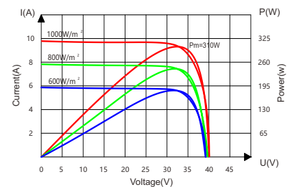
Current-Voltage&Power-Voltage Curve(310W)
