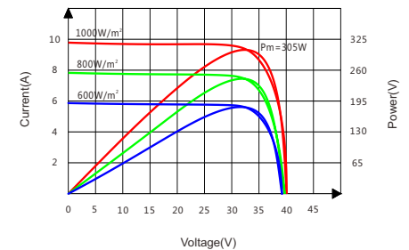
Current-Voltage&Power-Voltage Curve(305W)
